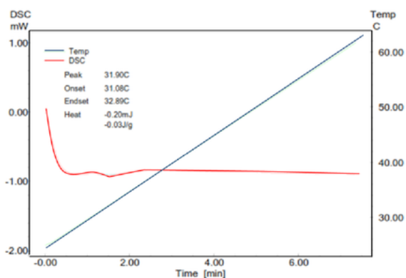
Fig. 2: DSC analysis of Celebes RBO
